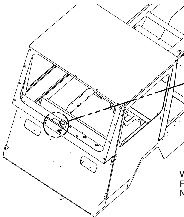
WINDSHIELD WIPER MOTOR & MOUNTING COMPONENTS
